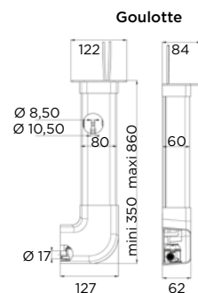
Sanicondens Clim pack
